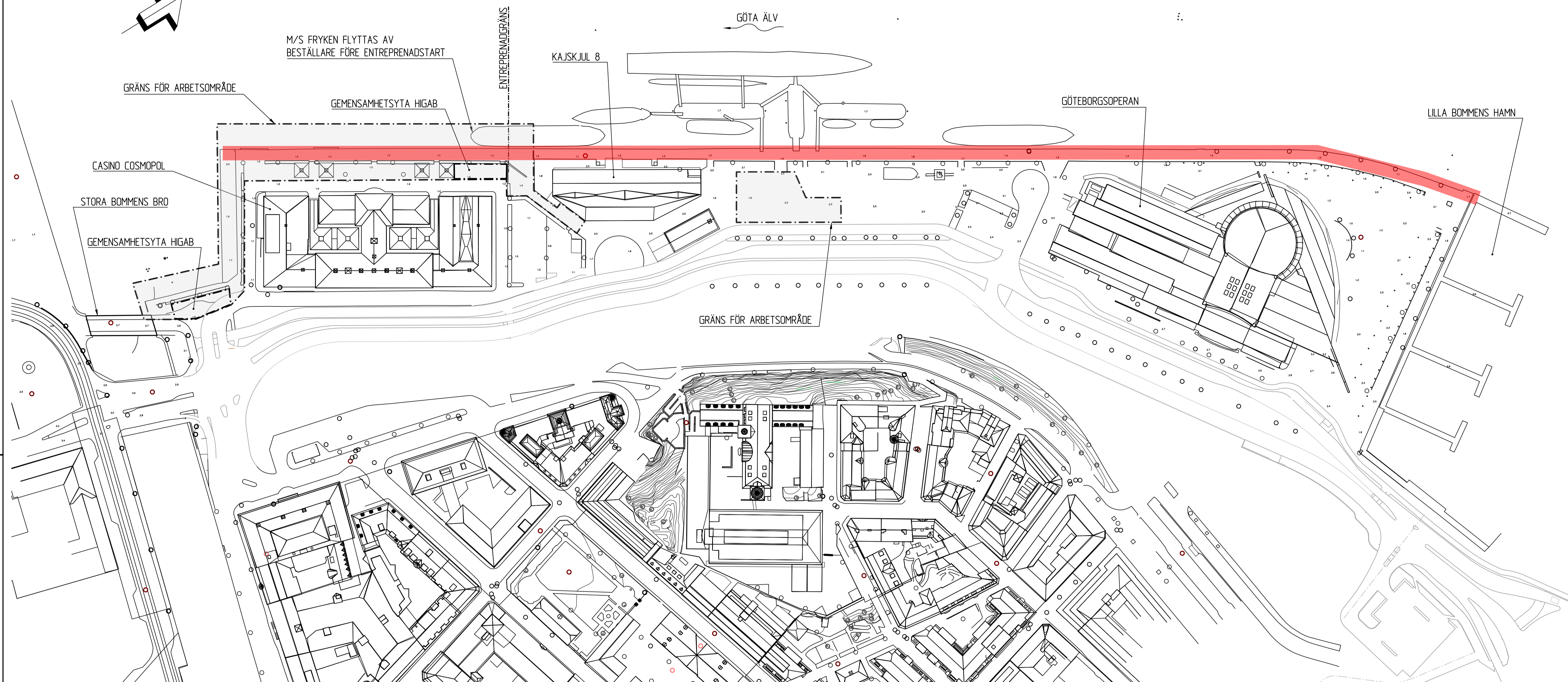
SITUATIONSPLAN 1:1000
